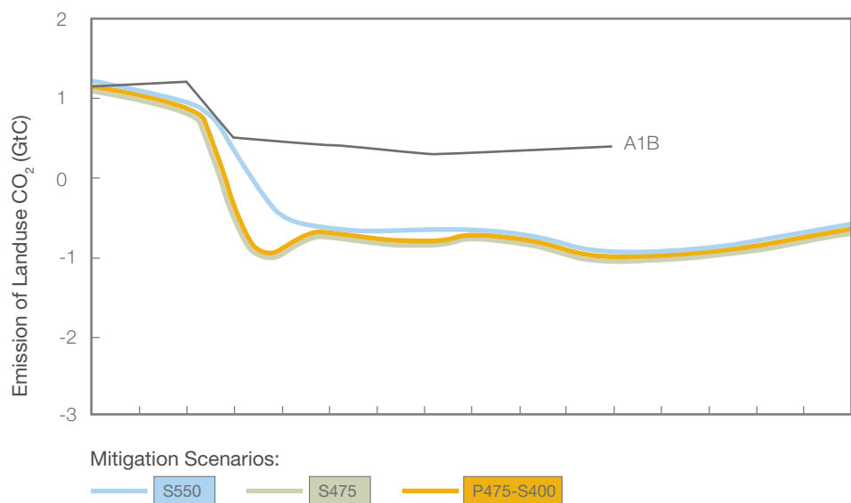
Figure 3. To permit a 500GtC carbon emissions budget, land-use emissions must be reduced over the period to 2050 as per the Meinhausen (2006) 400ppm scenario in the diagram. A failure to do so reduces the budget available to energy and other sectors.
