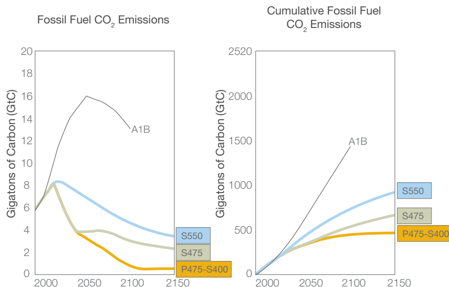
Figure 2. The diagram shows the trajectories of annual emissions and cumulative emissions in the Meinhausen (2006) 400ppm scenario as compared to various other scenarios.
