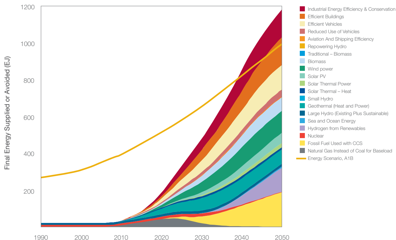
Figure 6. A representative scenario of the Climate Solutions Model depicting technology wedges capable of averting dangerous climate change. Each climate solution wedge grows over time and the sum of all wedges becomes significant as industrial capacity and deployment increase in scale. The top yellow line refers to the energy demand projection in the SRES A1B scenario. Note that since energy-efficiency technologies are shown alongside energy supply from low-emission sources, the results are expressed in final energy supplied or avoided (rather than primary energy production).
