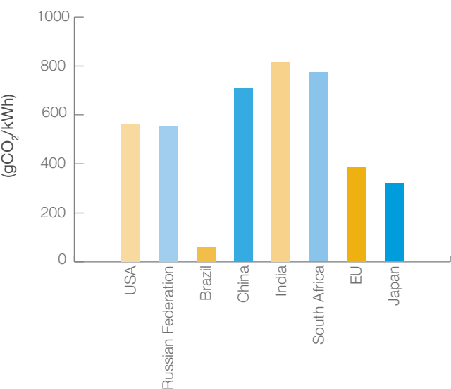
Carbon Intensity of Electricity Production
