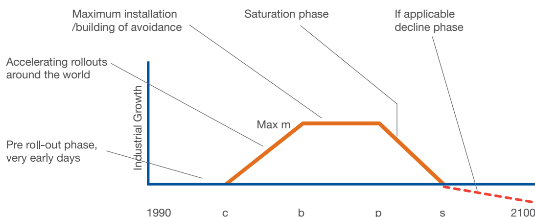
Figure 4. Trapezoid approximation for industrial growth. Any climate solution trapezoid can be fully defined by the set of variables c , b , p , s , and m .
