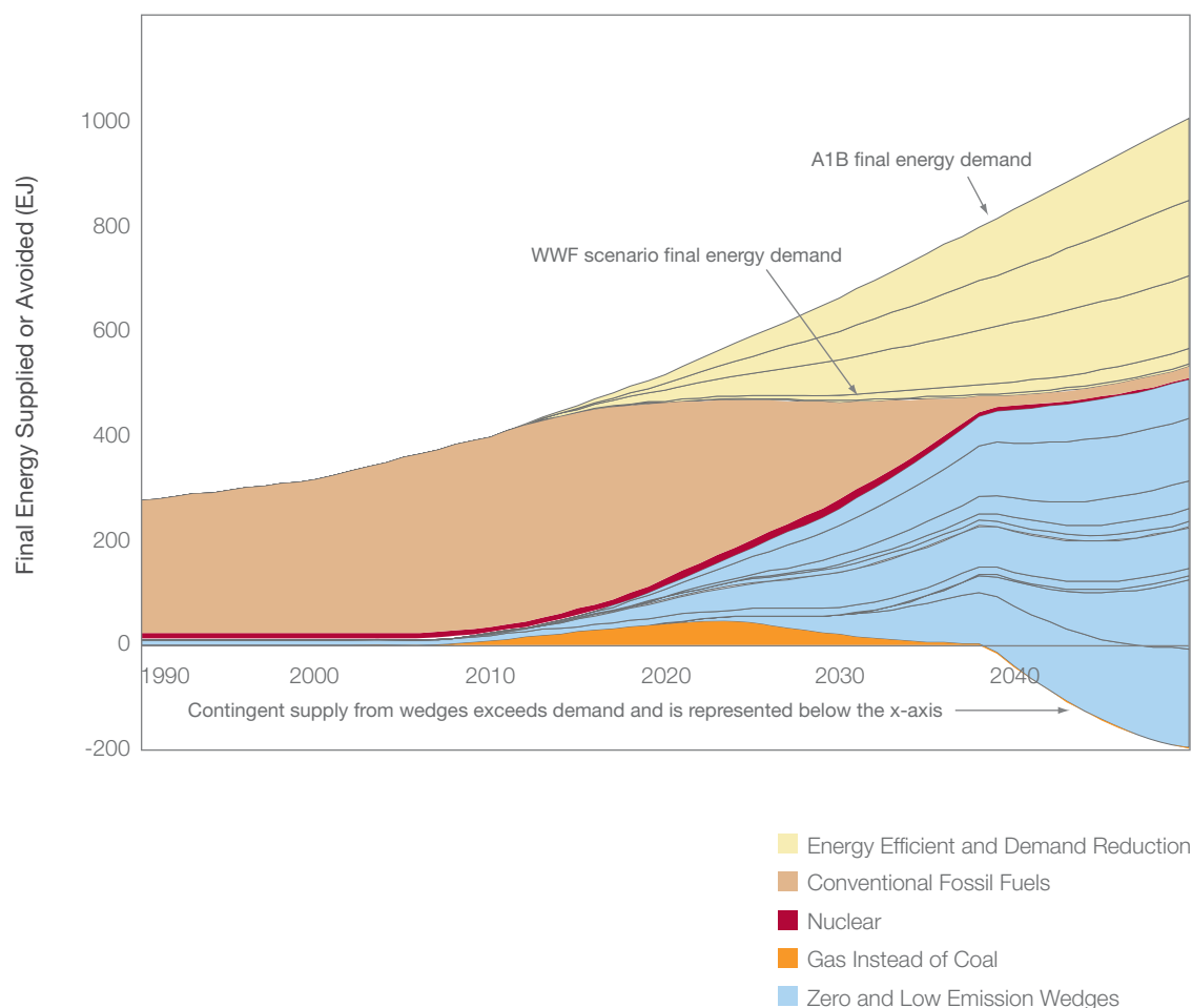
Figure 7. Output of the WWF Climate Solutions Model. Energy efficiency and demand reduction measures (drawing down from the top, in yellow) largely stabilize energy demand by about 2020, allowing a rising demand for the provision of energy services to be met from a more or less level supply of energy (notwithstanding regional variations). Meanwhile zero- and low-emission energy sources are built up (from the bottom, in blue) until about 2040 when, assuming none fail significantly, fossil-fuel use (in brown) is reduced to a "persistent" residual level of 20EJ for applications which are hard to replace. Nuclear energy use (in red) is phased out. It may of course be that some wedges under-perform or fail entirely. The scenario provides spare capacity as a contingency, represented by energy supply shown reaching below the x-axis.
