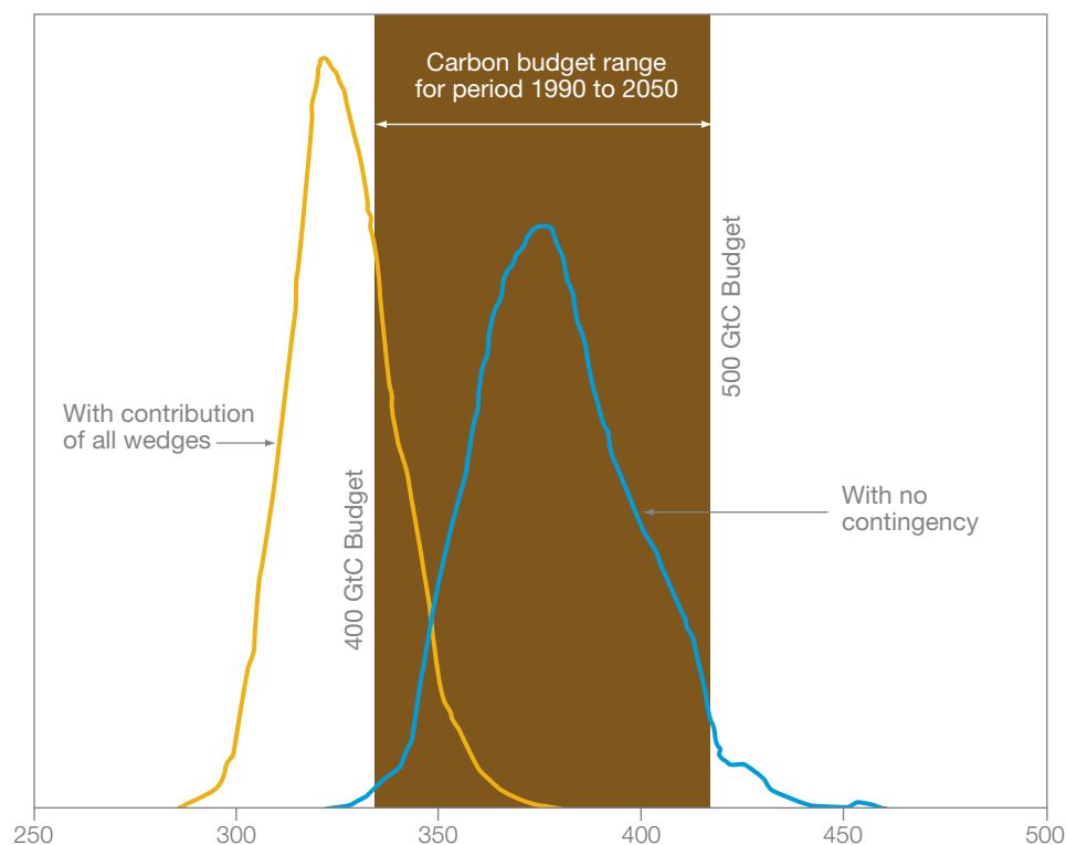
Carbon Budget Emissions for period 1990 to 2050 (GtC per year)
