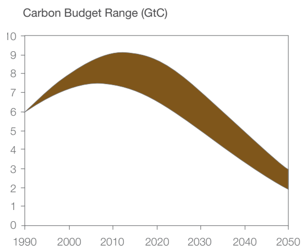
Figure 3. An indicative “carbon band”, showing the difference in the upper limits of annual allowable carbon emissions, from fossil fuels, in GtC per year, for total carbon budgets of 400GtC and 500GtC taken out to 2200 (showing the period to 2050 only). The thickness of the band therefore shows the crucial extra flexibility available in anthropogenic emissions if deforestation is successfully controlled.
