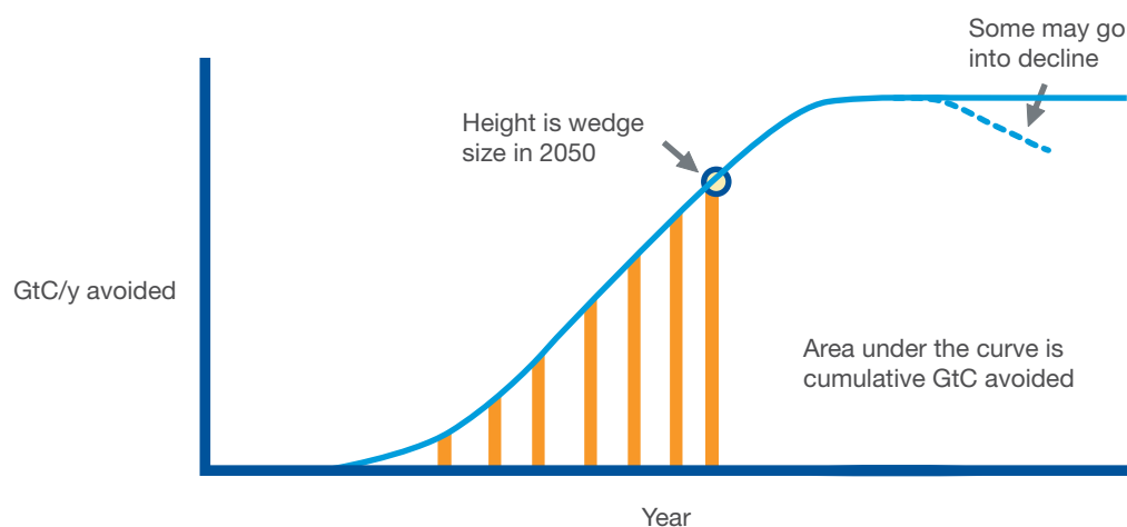
Figure 3. Emissions abated as a new technology grows.
