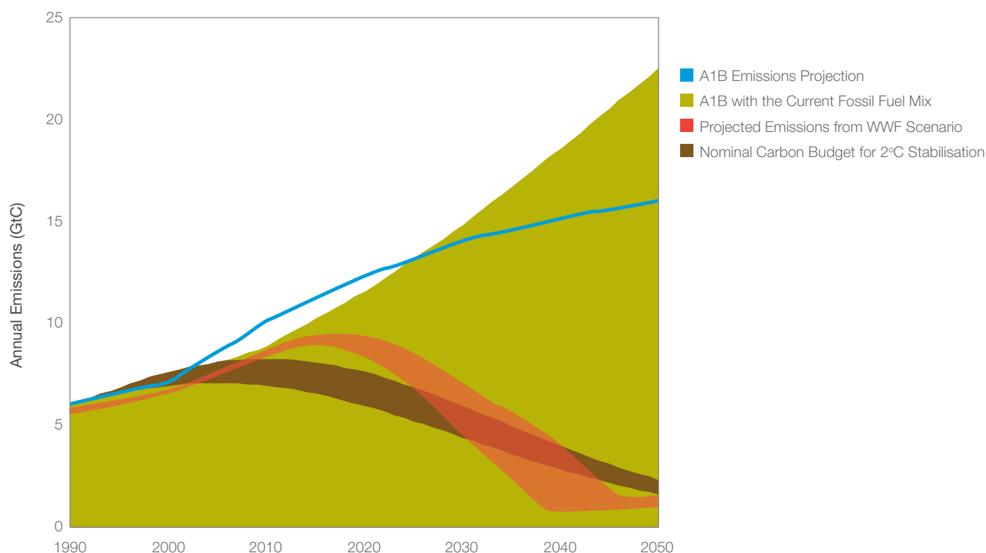
Figure 8. Emissions in the WWF Climate Solutions Model. The diagram shows the range of emissions (red bands) in the scenario presented in this paper. The lower limit of the red band shows the technical potential of emissions reduction if all wedges are fully implemented, and the whole “fossil fuel with CCS” wedge (yellow in Figure 6) comprises plants burning gas (which has lower carbon intensity). Emissions follow the upper limit line if about 80% of the potential is achieved and the “fossil fuel with CCS” wedge is made up of (higher carbon intensity) coal plants. Placed against the nominal carbon budget curve (brown), it is clear that the overall emissions to 2050 of the lower trajectory fall within the total emissions indicated by the upper limit of the budget range (assuming that deforestation is successfully brought under control). Any failure of efforts to halt deforestation (reducing the budget available for energy emissions to the lower limit of the brown band) will reduce the chances of staying within the overall emissions budget, especially if failures or delays in the implementation of solution wedges drive the emissions curve towards the upper limit of the red band. These curves are set against a backdrop (green) of the emissions that would occur if the IPCC’s A1B energy scenario were supplied with the current fossil-fuel mix (i.e., at about 0.02GtC/EJ). Also shown is the projected emissions curve for the A1B reference scenario which reaches annual emissions of 16GtC in 2050. The results of the modelling show that, although the point at which global emissions start to decline may not occur until 2015-2020, there is potential to drive deep cuts quickly once the industrial momentum behind transition is underway.
