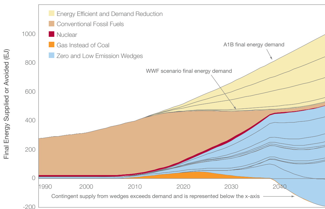
Figure 5. Output of the WWF Climate Solutions Model. Energy efficiency and demand reduction measures (drawing down from the top, in yellow) largely stabilize energy demand by about 2020, allowing a rising demand for the provision of energy services to be met from a more or less level supply of energy (notwithstanding regional variations). Meanwhile zero- and low-emission energy sources are built up (from the bottom, in blue) until about 2040 when, assuming none fail significantly, fossil-fuel use (in brown) is reduced to a “persistent” residual level of 20 EJ for applications which are hard to replace. Nuclear energy use (in red) is phased out. It may of course be that some wedges under-perform or fail entirely. The scenario provides spare capacity as a contingency, represented by energy supply shown reaching below the x-axis.
