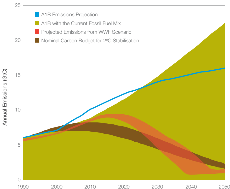
Figure 6. Emissions in the WWF Climate Solutions Model. The diagram shows the range of emissions (red bands) in the scenario presented in this paper. The lower limit of the red band shows the technical potential of emissions reduction if all wedges are fully implemented, and the whole “fossil fuel with CCS” wedge (yellow in Figure 4) comprises plants burning gas (which has lower carbon intensity). Emissions follow the upper limit line if about 80% of the potential is achieved and the “fossil fuel with CCS” wedge is made up of (higher carbon intensity) coal plants. Placed against the nominal carbon budget curve (brown), it is clear that the overall emissions to 2050 of the lower trajectory fall within the total emissions indicated by the upper limit of the budget range (assuming that deforestation is successfully brought under control). Any failure of efforts to halt deforestation (reducing the budget available for energy emissions to the lower limit of the brown band) will reduce the chances of staying within the overall emissions budget, especially if failures or delays in the implementation of solution wedges drive the emissions curve towards the upper limit of the red band. These curves are set against a backdrop (green) of the emissions that would occur if the IPCC’s A1B energy scenario were supplied with the current fossil-fuel mix (i.e., at about 0.02GtC/EJ). Also shown is the projected emissions curve for the A1B reference scenario which reaches annual emissions of 16GtC in 2050. The results of the modelling show that, although the point at which global emissions start to decline may not occur until 2015-2020, there is potential to drive deep cuts quickly once the industrial momentum behind transition is underway.
