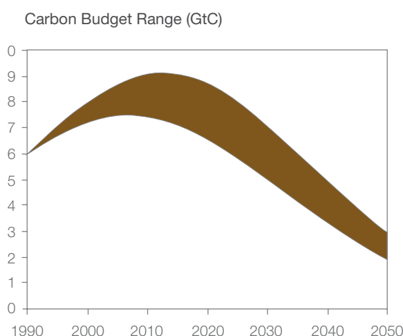
Figure 1. An indicative “carbon band”, showing the difference in the upper limits of annual allowable carbon emissions, from fossil fuels, in GtC per year, for total carbon budgets of 400GtC and 500GtC taken out to 2200 (showing the period to 2050 only). The thickness of the band shows the crucial extra flexibility available in anthropogenic emissions if deforestation is successfully controlled.
