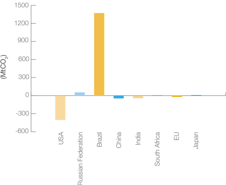
Greenhouse Emissions from Land Use Change and Forestry
