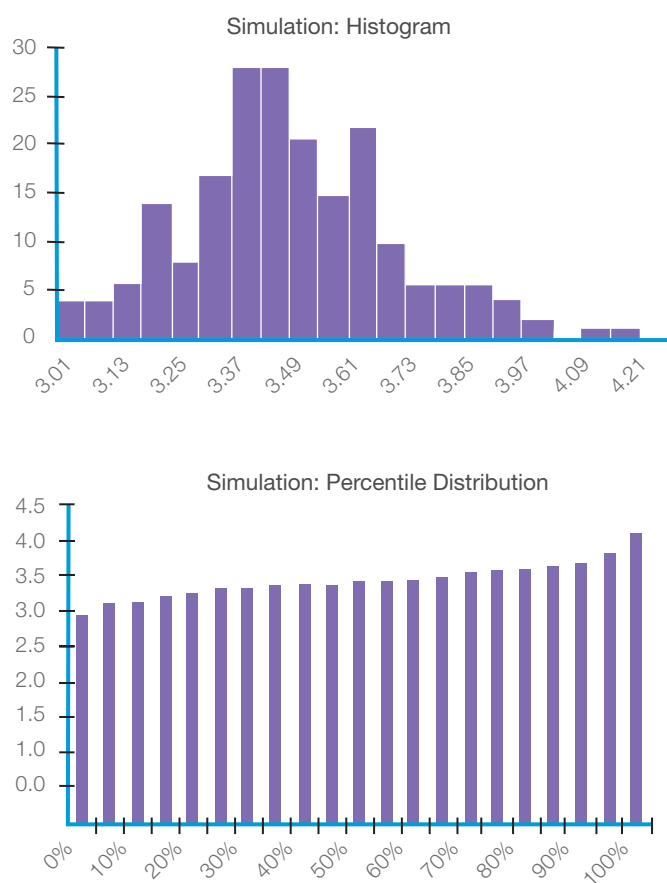
Figure 5. Example distribution for an output for a sample run of the model, presented as a histogram and percentile distribution. These indicate the range of possible outcomes, the most likely outcome and a probability distribution for any given output.
